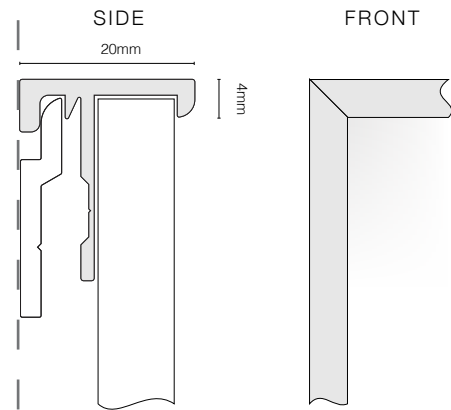
FLAT TO THE WALL MOUNTING
